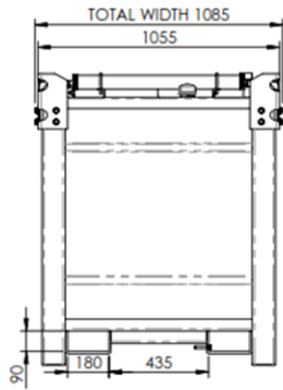
ELEVATION VIEW
