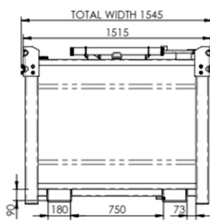
ELEVATION VIEW
