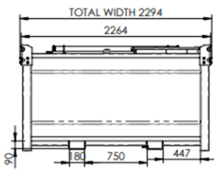
ELEVATION VIEW
