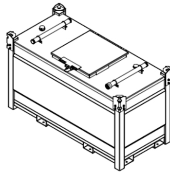
ISOMETRIC VIEW 1
