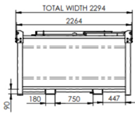
ELEVATION VIEW
