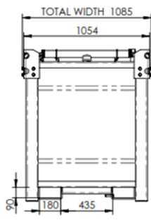
ELEVATION VIEW
