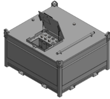
ISOMETRIC VIEW 2
