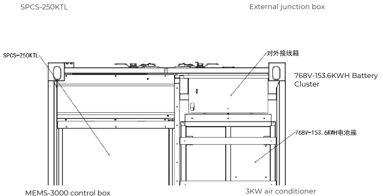
Figure 5-9: System Arrangement
