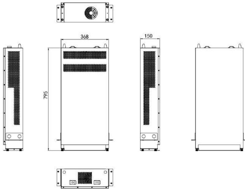
Figure 5-2: Battery Module
