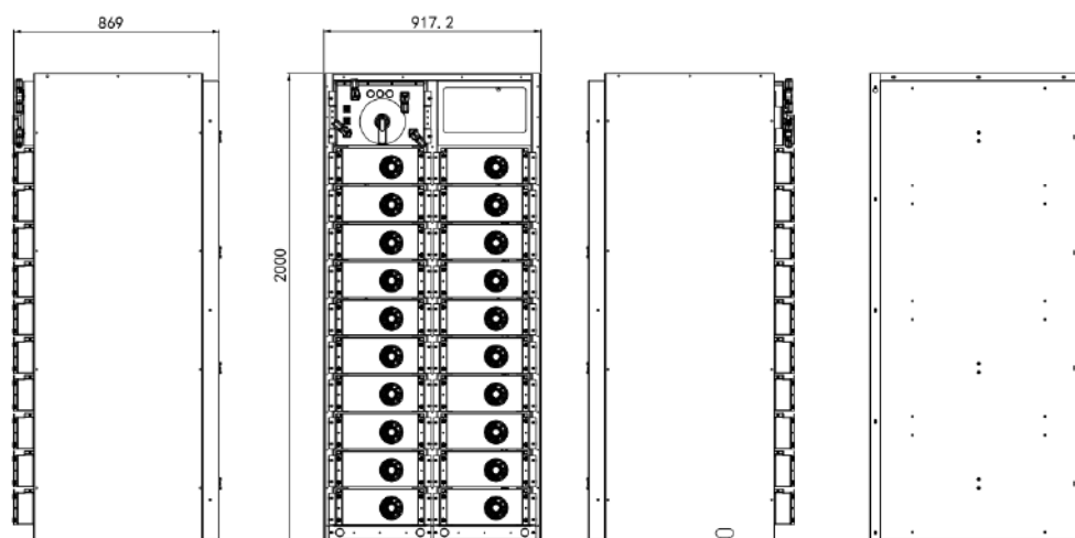
Figure 5-3: Battery Cabinet
